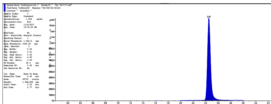
Figure 5. Chromatogram of stock solution of internal standard Caffeine Solution with Plasma
