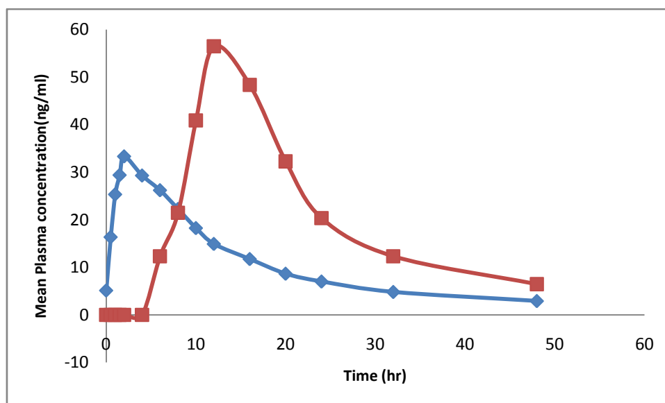
Figure: 4. Concentration-Time Curve of Azathioprine following of core-in-cup tablets and pure drug
