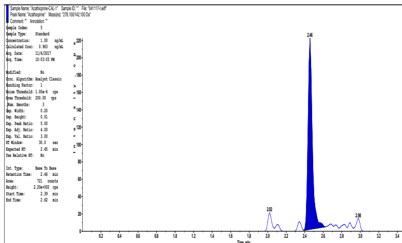
Figure 4. Chromatogram of stock solution of Standard Azathioprine Solution with Plasma
