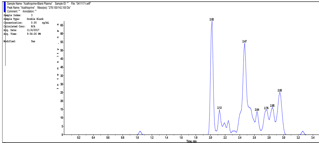
Figure 2. Chromatograms of blank Plasma
