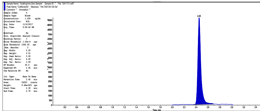
Figure 3. Chromatograms of blank and internal standard
