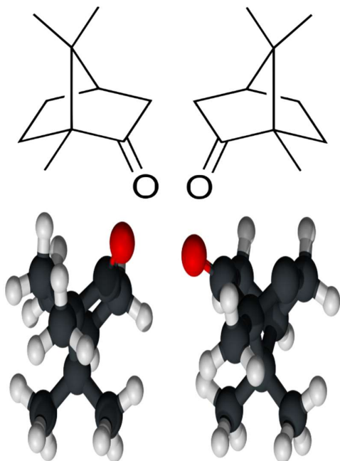
1, 7, 7-Trimethylbicyclo [2.2.1]heptan-2-one
