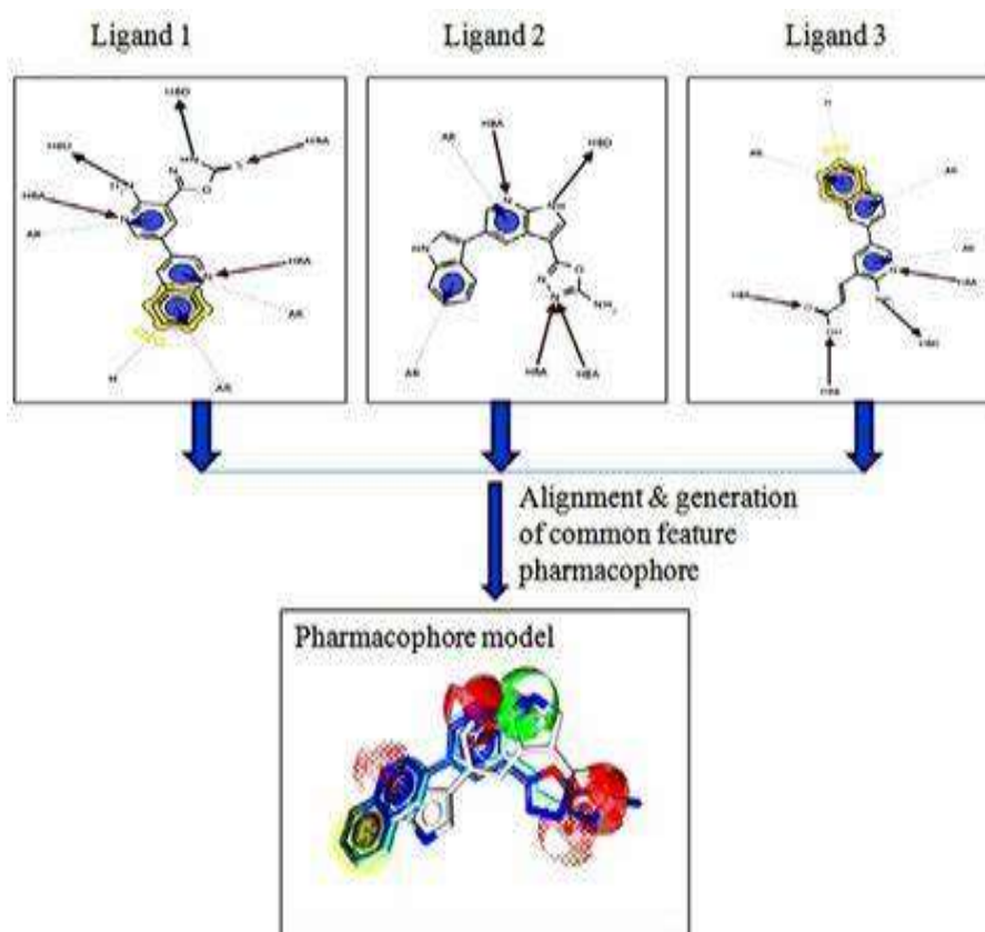
Fig. Ligand-based pharmacophore modeling.
