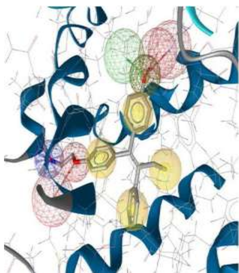
Figure 2: 3D Structure based pharmacophore modeling.[18]
