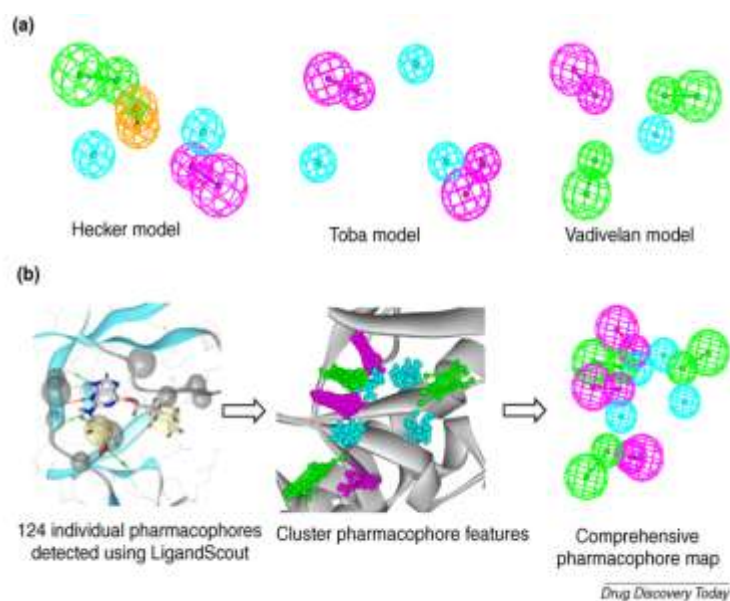
Fig: Pharmacophore models of cyclin-dependent kinase 2 (CDK2) inhibitors. (a) Pharmacophore models of CDK2 inhibitors developed using Catalyst by Hecker et al. [24], Toba et al. [25] and Vadivelan et al. [26]. (b) The basic process for the generation of multicompound-based comprehensive pharmacophore map of CDK2 inhibitors. The chemical features are color coded: green, hydrogen-bond acceptor; magenta, hydrogen-bond donor; light blue, hydrophobic feature; orange, aromatic ring.
