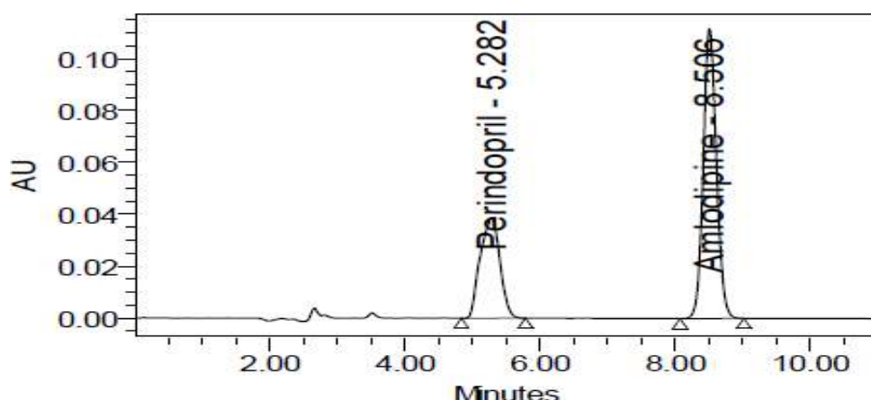
Fig. 1: Typical chromatogram of perindopril and amlodipine
