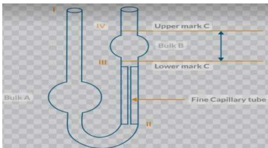
Figure 4.8: OSTWALD VISCOMETER
