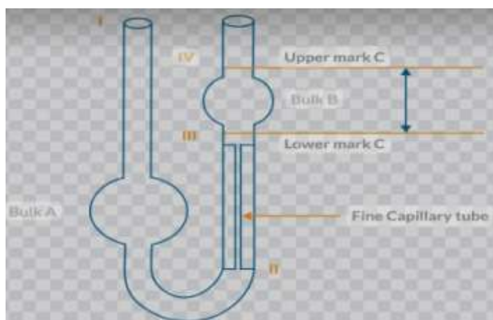
Figure 4.8: OSTWALD VISCOMETER
