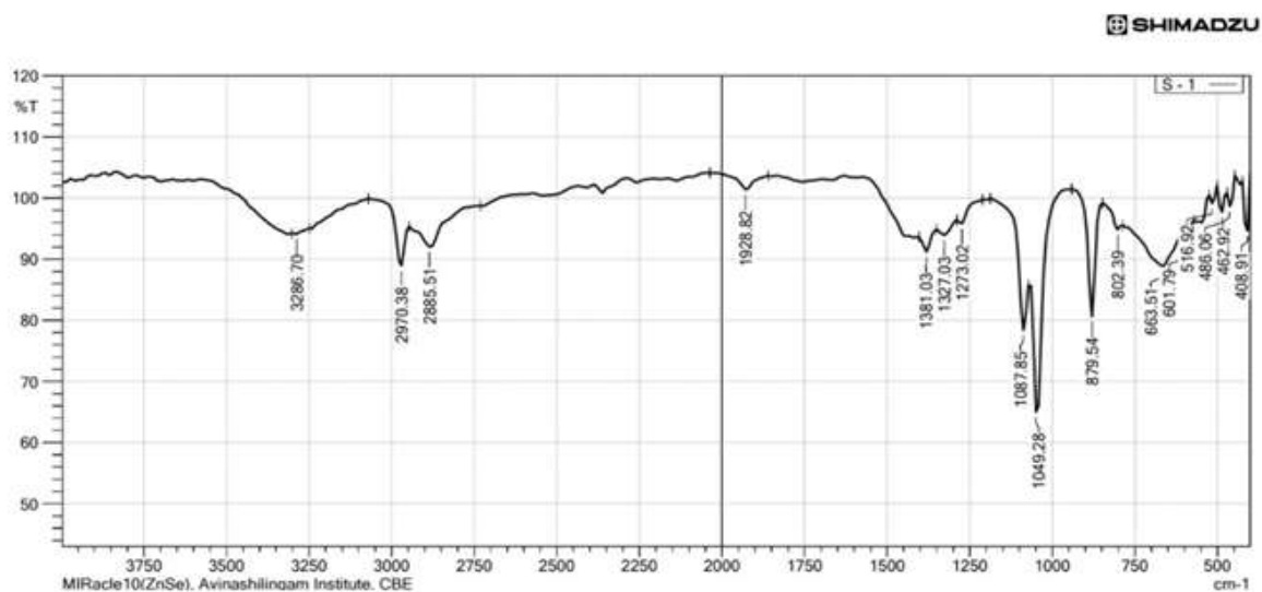
Fig 1: FT-IR Analysis of Copper Nano Particles
