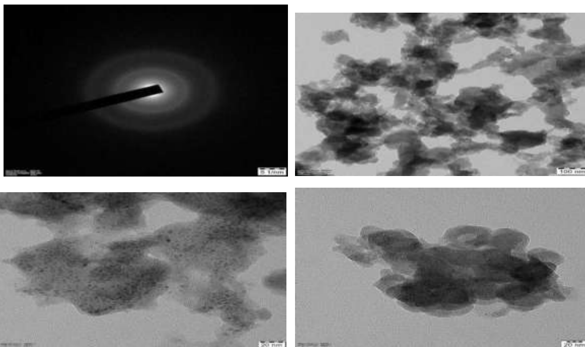
Fig 4: TEM images of green synthesised copper nanoparticles at lower magnification (100nm) and
