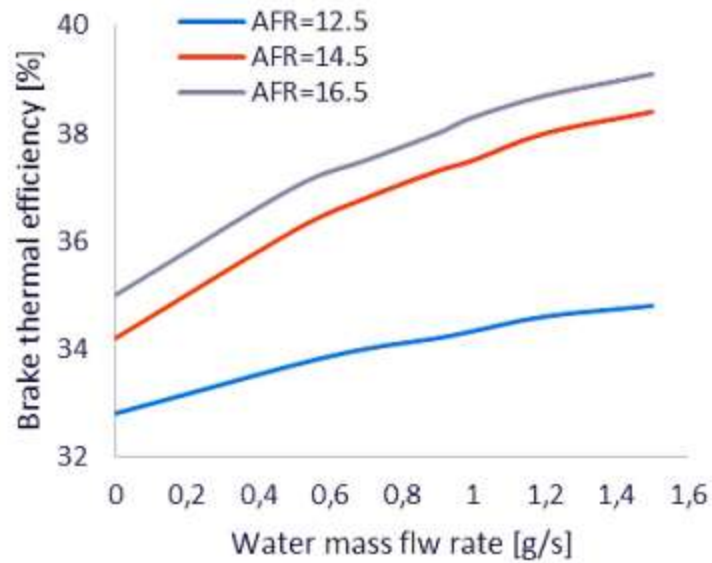
Figure 2. Effect of water injection on engine thermal efficiency [4]
