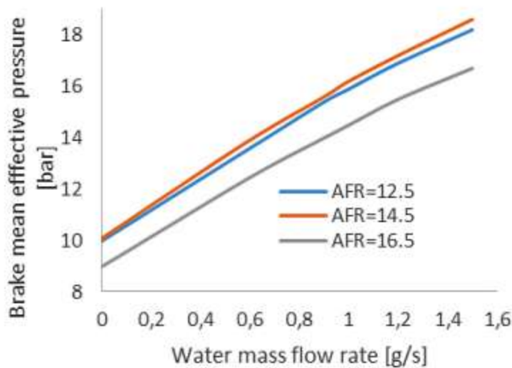
Figure 5. Effect of water injection on engine pressure [4]
