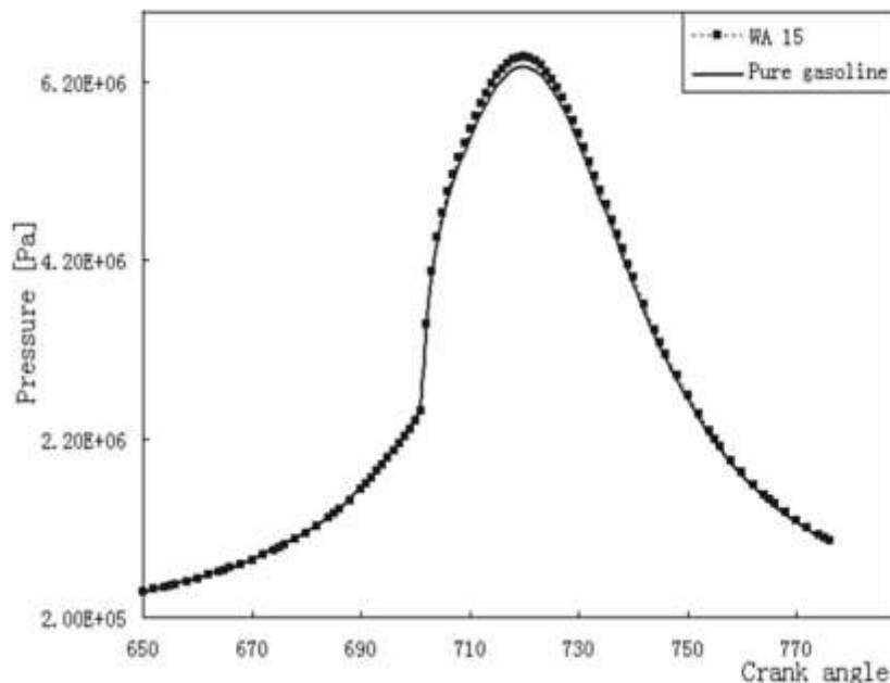
Figure 7. The increase of peak in-cylinder pressure for the volumetric expansion of steam. [N2]
