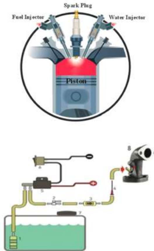
Figure 1. Schematic of water injection implementation; 1) water filter; 2) one way valve; 3) one way filter, 4) orifice; 5) vacuum solenoid; 6) on/off switch; 7) water tank; 8) intake manifold [5]
