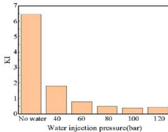
Figure 9. KI (Knocking) under different injection pressures [6]
