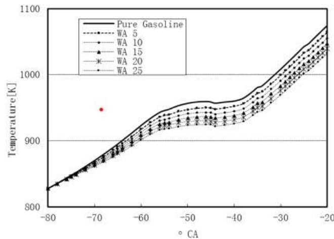
Figure 6. The decrease in compressed charge temperature as a consequence of injected water [N2]
