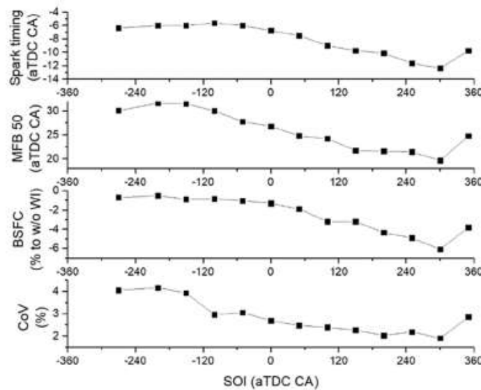
Figure 10. Water injection timing effect on combustion characteristics and fuel consumption. Engine speed of 1600 RPM, BMEP of 7 bar, injection pressure of 100 bar, WFR of 0.47 [8]
