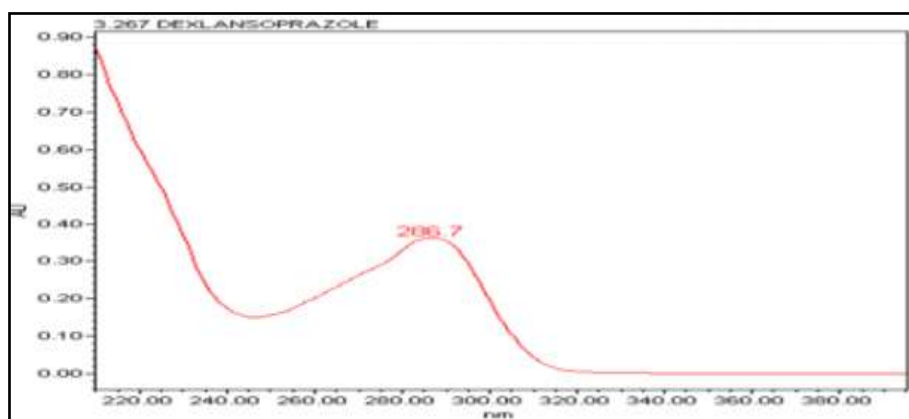
Fig. 1: UV Spectrum of Dexlansoprazole
