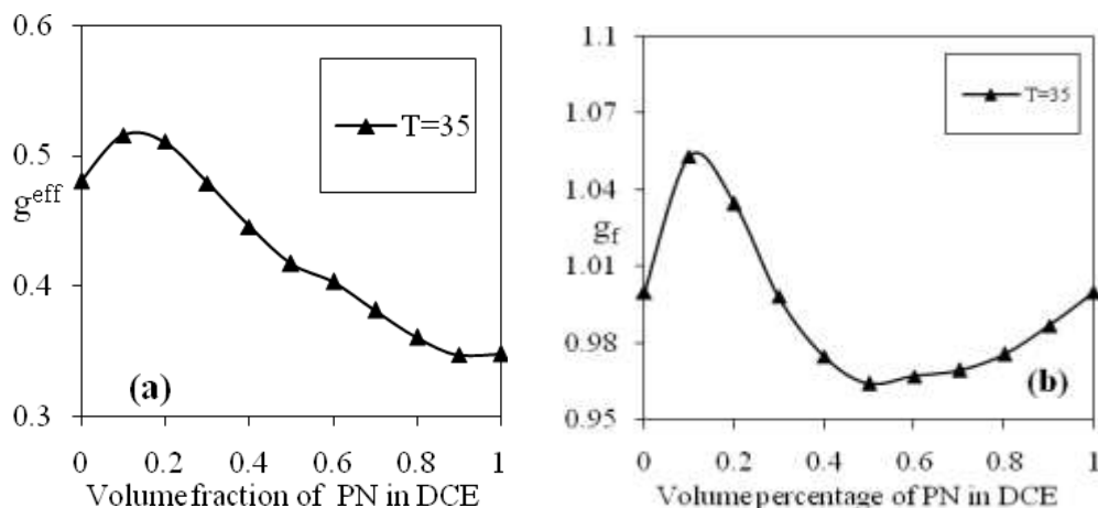
Figure1. (a) Kirkwood effective correlation factor g^{eff} and (b) Kirkwood correlation factor g_f , versus volume fraction (□□□ of PN in DCE.
